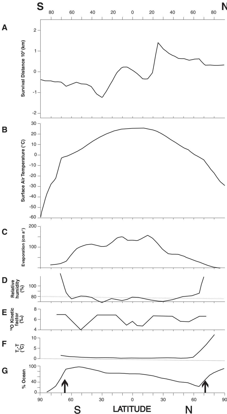
FIGURE 5. Modern annual zonal averages of annual input data fields for the isotope model, and model output compared to observations (Fisher, 1990). (A) Survival distance (km) for water vapour (l). Positive values indicate northward vapour transport. (B) Near-surface air temperature (T). (C) Evaporation rate (E). (D) Near-surface relative humidity (h). (E) Kinetic evaporation fractionation factor ( k_{18} ). (F) Difference between the sea temperature and the air temperature ( T_c - T ). (G) Percentage of the zone that is ocean with vertical arrows indicating the annual average position of the sea ice.
