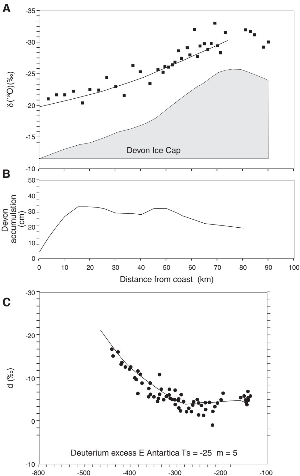
FIGURE 7. Example of the regional model for the southeast side of the Devon Ice Cap. (A) The \delta(^{18}O) data (squares) and (B) the accumulation rate data (both from Koerner and Russell, 1979). The lines are predicted by the model (Fisher, 1992) using the measured accumulation and coastal values of \delta(^{18}O) . (C) An East Antarctic example of d versus \delta(^{18}O) from observations (Petit et al. , 1991). The line is that predicted by the regional model (Fisher, 1992).
