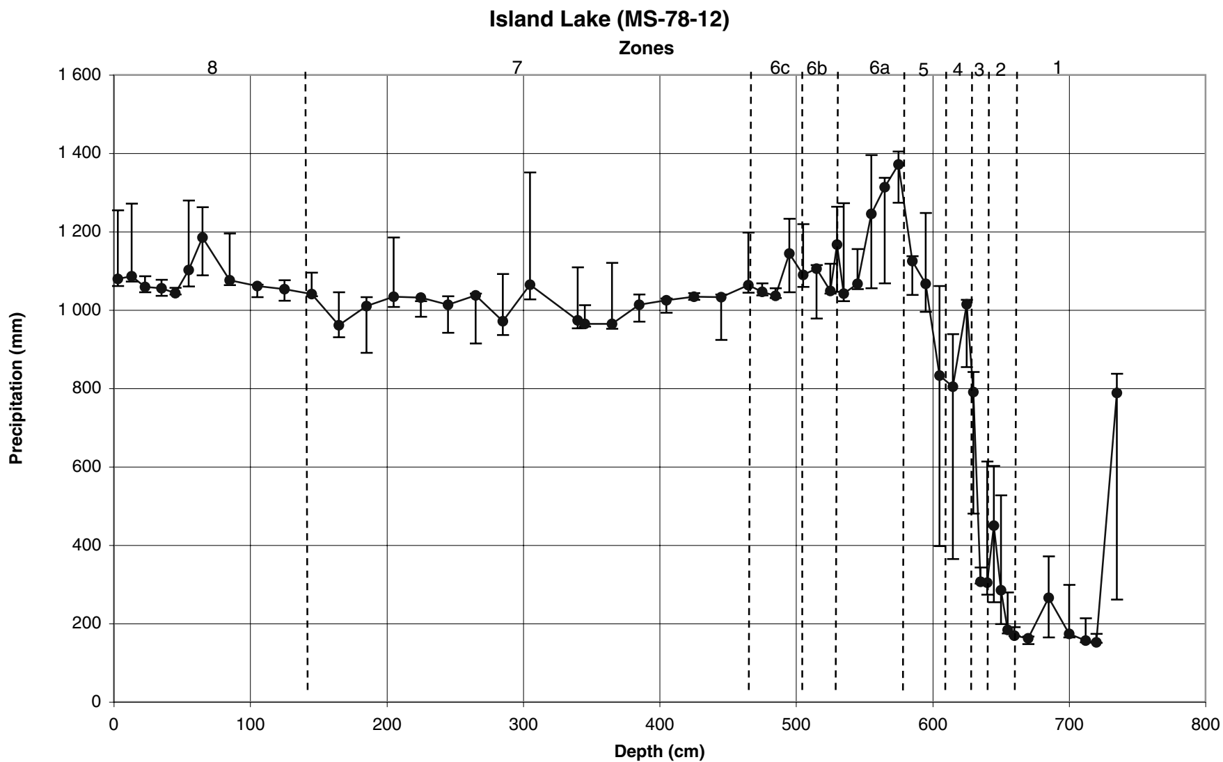
Figure 3B. Island Lake precipitation reconstruction.
