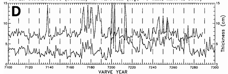
UPPER CONNECTICUT (bottom) vs. WINOOSKI (top, +4 cms; Antevs, 1928)
