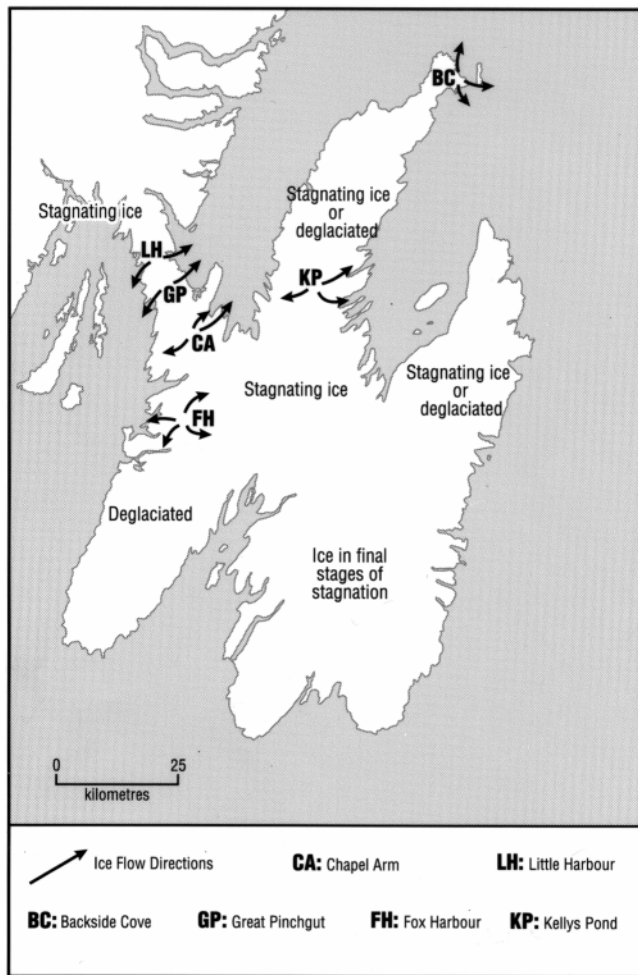
FIGURE 16. Ice Centres and Flow Directions during the final stages of deglaciation. Ice flow directions are based on striations and streamlined landforms documented in Catto (1992a, 1993, 1994a, b), and Taylor et al. (1994).
