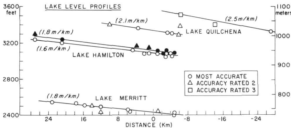
FIGURE 12. Isostatic deformation of glacial lake strandlines in the Nicola River basin, Thompson Plateau. Solid symbols are used for shore features related to the upper level of Lake Hamilton (from Fulton and Walcott, 1975).
