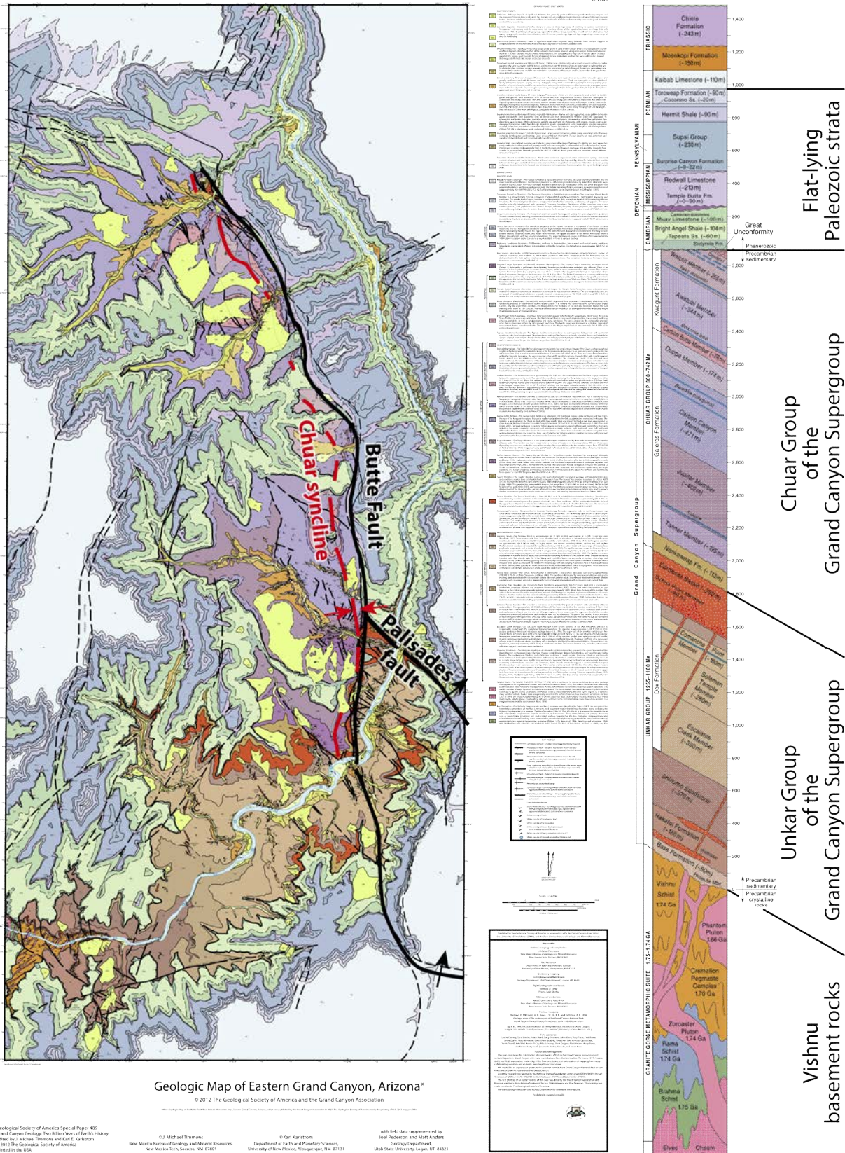
Figure 9. Timmons and Karlstrom (2012) Geologic map of Eastern Grand Canyon, Arizona showing updated rock column (from sheet 2, on backside). This map and the accompanying Geological Society of America Special Papers v. 489 are available as pdfs from the Geological Society of America ( https://rock.geosociety.org/Store/detail.aspx?id=SPE489P ).
