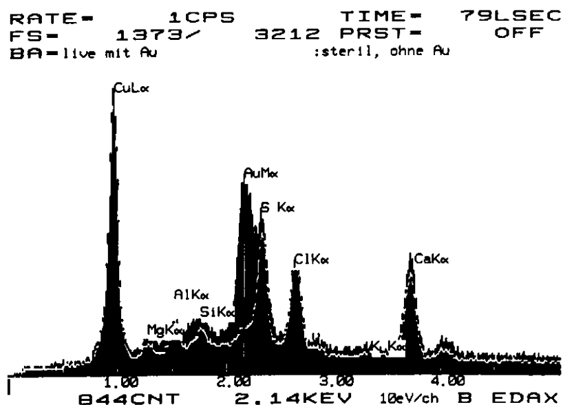
Figure 1 Energy dispersive X-ray microanalysis, at 2.14 KEV, of elements in the glycolyx of a filament of Plectonema terebrans . The solid curve filled in black shows results of analysis of live cultures incubated in gold solution; notice the peak for gold. The superimposed white curve shows results from heat-killed cultures in gold solution. The two curves are similar except for the absence of gold in the heat-killed microorganisms. The analysis was made at a rate of 1 count per second for 79 seconds. (From Dyer et al. , 1994, with permission)
