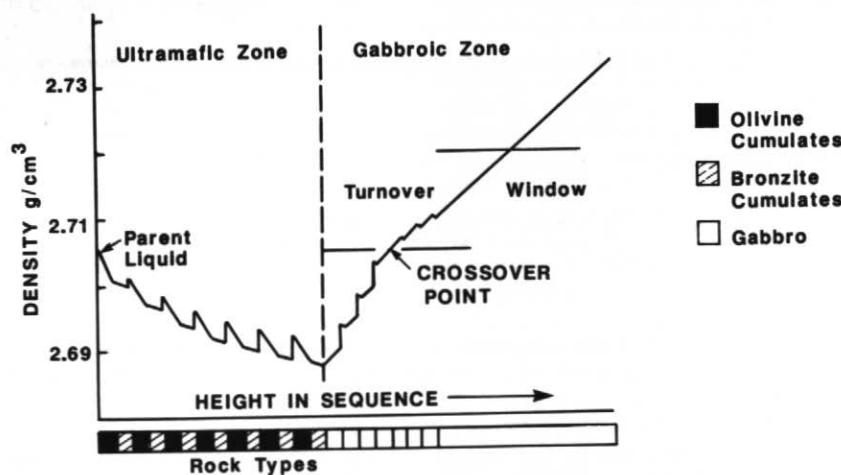
Figure 8 Density variation of magma during sequential injection of primitive melts. Each cyclic unit is assumed to mark the introduction of a new pulse of magma into the chamber equal to 25% of the volume of the magma in the chamber. The turnover window is the density range in the fractionated magma for which magma turnover is possible (after Campbell et al. , 1983).
