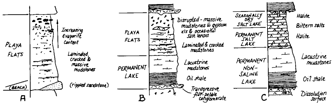
Figure 6 Hypothetical cycles reflecting increasing aridity. A: Distal playa flats. B: Playa flats marginal to playa lake. C: Playa lake
