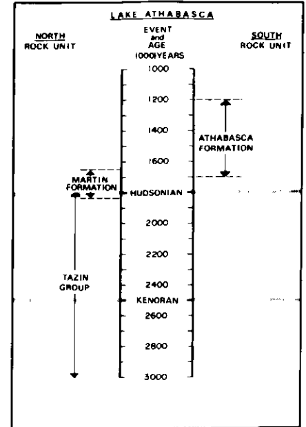
Figure 11 Rock units of the Athabasca Region (Dates after Fraser, 1970).
