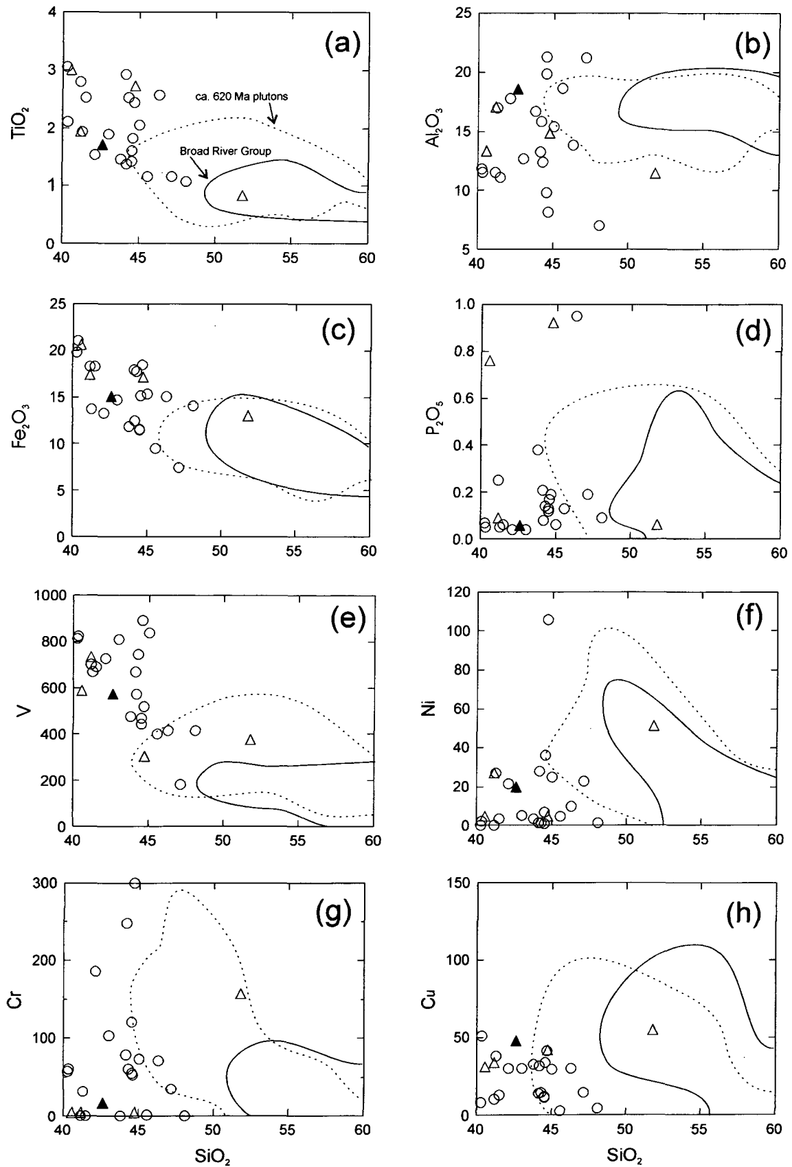
Fig. 4. Selected silica variation diagrams to illustrate chemical characteristics of the Caledonia Mountain Pluton. Circles are data from Blackwood (1991), open triangles are data from Barr and White (1999), and black triangle is dated sample CM97-1 (data in Table 2). Solid line field encloses data from volcanic rocks with less than 60% \text{SiO}_2 in the ca. 600-625 Ma Broad River Group ( n = 59 ), and dashed line field encloses data from associated ca. 615-620 Ma plutons with less than 60% \text{SiO}_2 ( n = 21 ) derived from data in Barr and White (1999).
