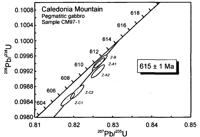
Fig. 3. U-Pb concordia diagram for zircon fractions from the Caledonia Mountain gabbro (sample CM97-1). Shaded ellipse (fraction A2) is excluded from the age regression. Data are from Table 1.
