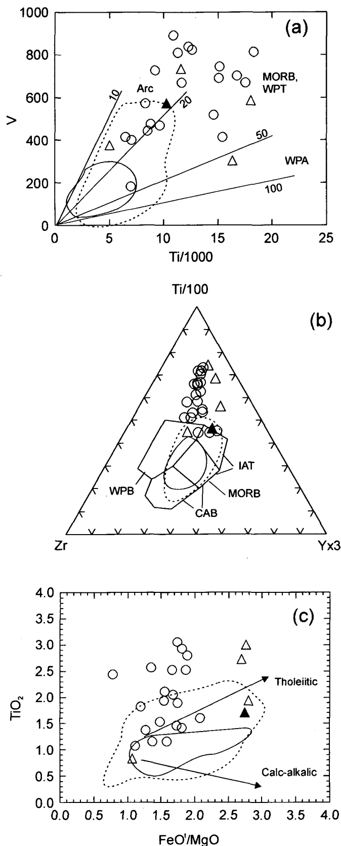
Fig. 5. Plots of (a) V-Ti, (b) Ti-Zr-Y, and (c) \text{TiO}_2 - \text{FeO}/\text{MgO} for data from the Caledonia Mountain gabbro with symbols and solid and dashed line fields as in Fig. 4. Labeled fields in (a) and (b) and trends in (c) are from Shervais (1982), Pearce and Cann (1973), and Miyashiro (1974), respectively. Abbreviations: MORB, mid-ocean ridge basalt; WPT, within-plate tholeiitic basalt; WPA, within-plate alkalic basalt; IAT, island-arc tholeiite; CAB, calc-alkalic basalt; WPB, within-plate basalt.
