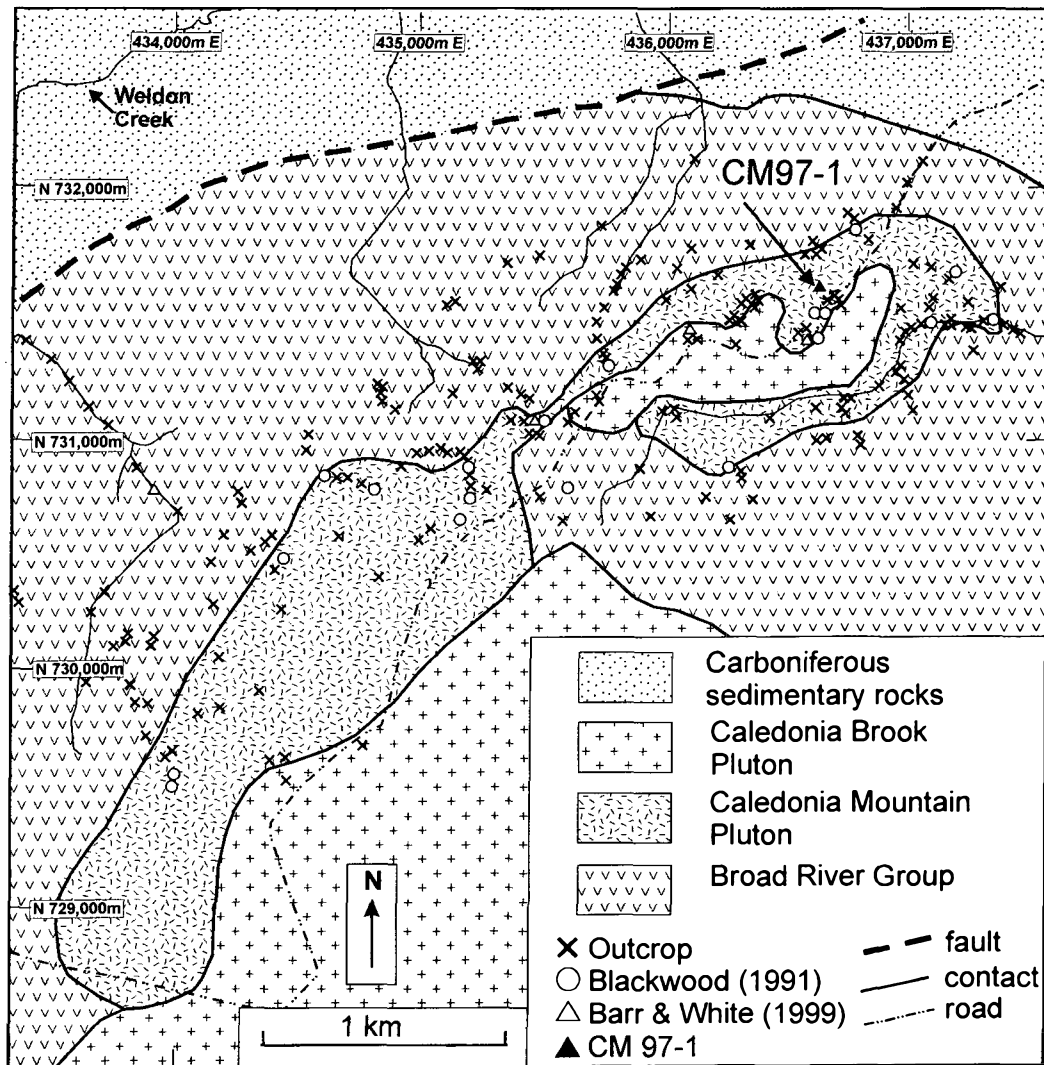
Fig. 2. Geological map of the Caledonia Mountain Pluton and surrounding area showing sample locations from Blackwood (1991) and Barr and White (1999). Outcrops (x) were compiled from Blackwood and Cormier (1990) and Barr and White (1993). Locations of analyzed samples of Blackwood (1991) were inferred from data in Blackwood and Cormier (1990) and Blackwood (1991). CM97-1 is the dated sample.
