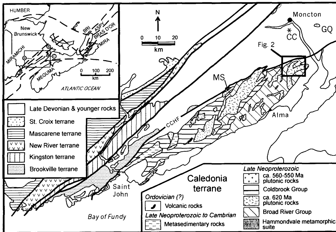
Fig. 1. Simplified geological map of the Caledonia Highlands (after Barr and White 1999), showing the location of the Caledonia Mountain Pluton and other units referred to in the text. CC, GQ, and MS indicate the locations of the Lower Coverdale ferrogabbro complex, the Gaytons quarry, and the Mechanic Settlement Pluton, respectively. CCHF is the Caledonia-Clover Hill fault. Inset map shows the location of the map area in southern New Brunswick in relation to terranes of Barr and White (1996b); BRI, Blair River inlier, C, Caledonia terrane, B, Brookville terrane, and N, New River terrane.
