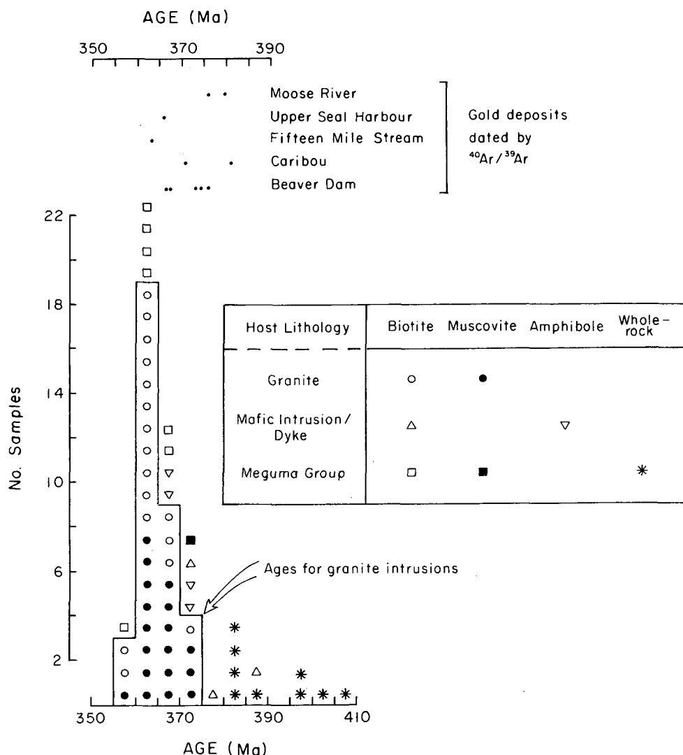
Fig. 16. Histogram plot of 40 Ar/ 39 Ar ages for granites, mafic intrusions and Meguma Group metasedimentary rocks in the eastern Meguma Terrane. Sources of data: Reynolds et al. (1981), Keppie and Dallmeyer (1987), Kempster et al. (1989), Kontak et al. (1989a, 1990a). Ages for the gold deposits are from this study. Note that in addition to the ages shown, Krogh and Keppie (1988) reported U/Pb zircon and monazite ages of ca. 372 Ma for the Larrys River and Halfway Cove plutons of the eastern Meguma Terrane.
