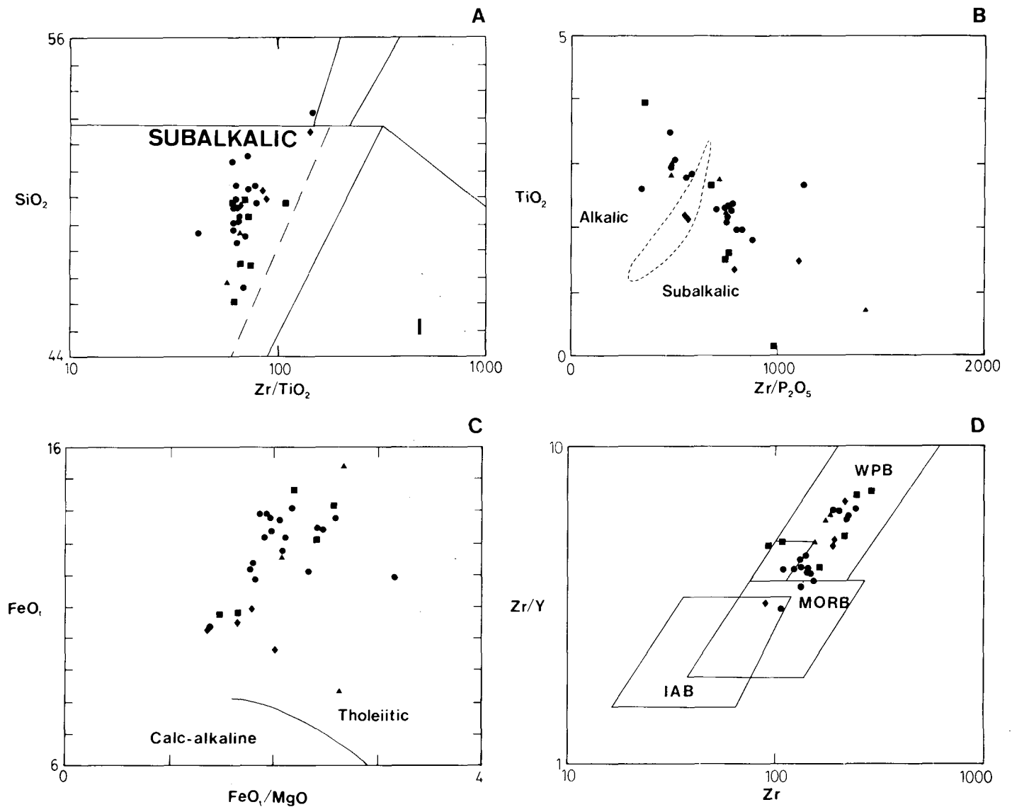
Fig. 4. Petrogenetic affinity of the mafic rocks of the Folly River Formation. (A) after Winchester and Floyd, 1977. (B) after Floyd and Winchester, 1975. (C) after Miyashiro, 1974. (D) after Pearce and Norry, 1979. Solid circles represent the volcanic rocks from the Folly River Formation in the Debert River area and those interlayered with turbidites. Triangles represent dykes cutting the Gamble Brook Formation. Squares represent dykes within the Great Village River Gneiss. Crosses represent the dykes cutting the volcanic rocks of the Folly River Formation.
