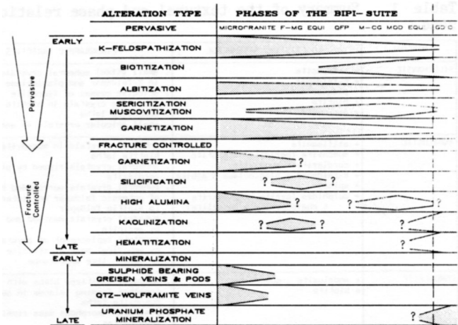
Fig. 2. Chronological sequence of alteration and mineralization types within the BIPI suite. Alteration exhibits transition in style from early pervasive to later fracture controlled. The unit in which the alteration is observed is also displayed; the units are listed beginning with the latest intrusive(?) unit (microgranite). The wider the bar the more intense the particular type of alteration.
