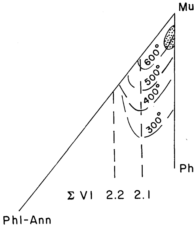
Fig. 9. Muscovites of the HAHA zone (shaded area) plotted on the \Sigma VI versus Si cation diagram of Monier and Robert (1986). Isotherms are shown by dashed (long) lines.
