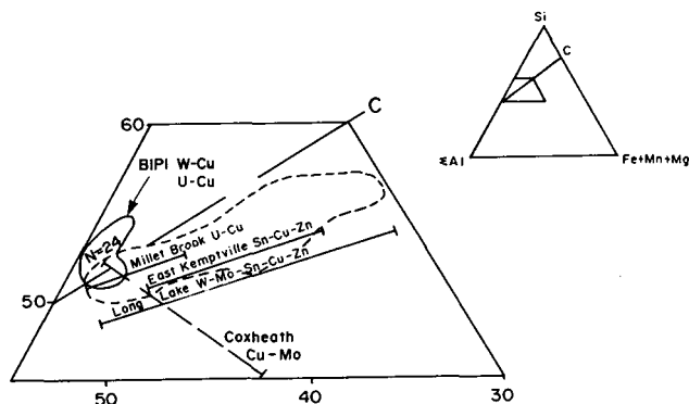
Fig. 4. Muscovite compositions from the HAHA zone plotted in the \Sigma\text{Al-Si-(Fe+Mn+Mg)} diagram (modified from Kontak and Corey, in press). Analyses are compared to muscovites analyzed by Strong and Chatterjee (1985) from other hydrothermal mineral deposits within Nova Scotia (enclosed by heavy dashed line).
