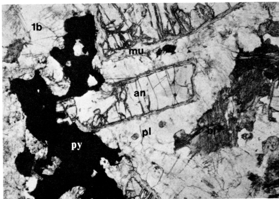
Plate 1b. Euhedral andalusite crystal exhibiting a sericitic alteration rim and feldspar halo is partially enveloped by late-stage pyrite (opaque). Field of view is 1 mm.
