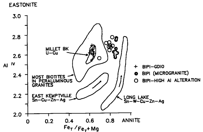
Fig. 7. Al iv over Fe/(Fe+Mg) plot for biotites from the BIPI suite. Comparisons are made to Clarke's (1981) field for biotites in peraluminous granites and also those defined by Strong and Chatterjee (1985) for biotites from other hydrothermal mineral deposits within the SMB.
