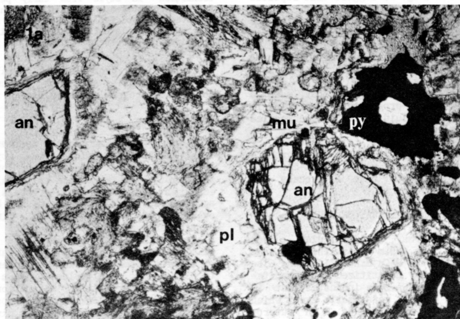
Plate 1a. Andalusite crystals surrounded by bleached halo composed of oligoclase ( An_{11}-An_{16} ). Clustered around the perimeter are masses of pinite and biotite. Field of view is 1 mm. an: andalusite, mu: muscovite, pl: plagioclase, py: pyrite.
