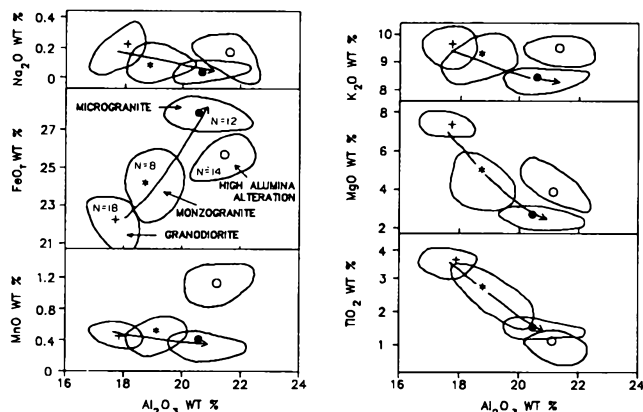
Fig. 5. Oxide wt.% contents of biotites from units of the BIPI suite versus their Al 2 O 3 wt.%. Symbol location represents average analyses for units, whereas variation within each unit is denoted by circle surrounding symbol. Arrows represent assumed magmatic/metamorphic trends.
