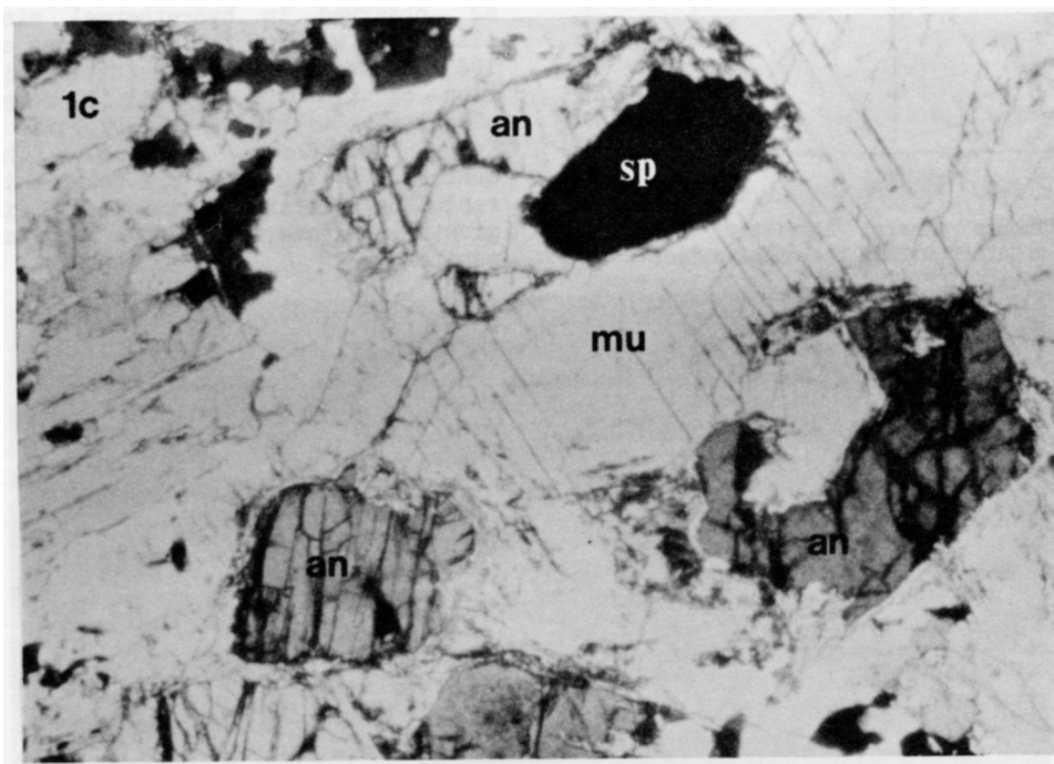
Plate 1c. Small (<1 mm) hercynite-spinel grain (isotropic) occupying core of andalusite crystal. Field of view is 0.4 mm. sp: spinel
