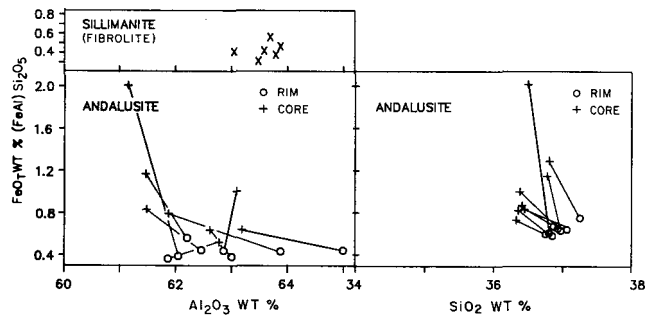
Fig. 3. Aluminosilicate mineral chemistry; note the strong (FeAl)Si 2 O 5 zonation within the andalusites.
