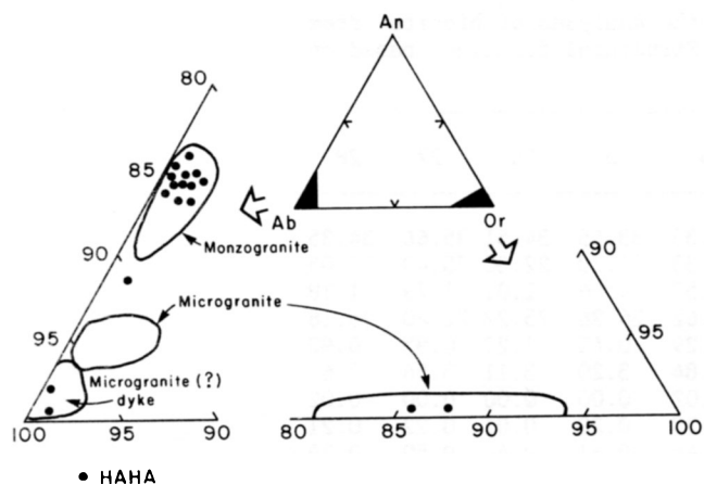
Fig. 8. Composition of feldspars from the HAHA zone (solid dots) plotted in the An-Ab-Or diagram. Data is compared to fields delineated by Kontak and Corey (in press) for several units of the BIPI suite.
