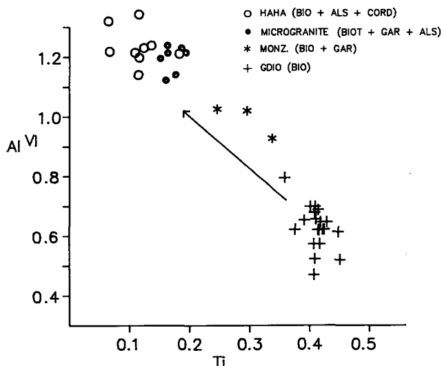
Fig. 6. Al vi versus Ti plot (adapted from LeBel, 1979), for biotites from the BIPI suite. Arrow shows decreasing temperature of biotite crystallization.
