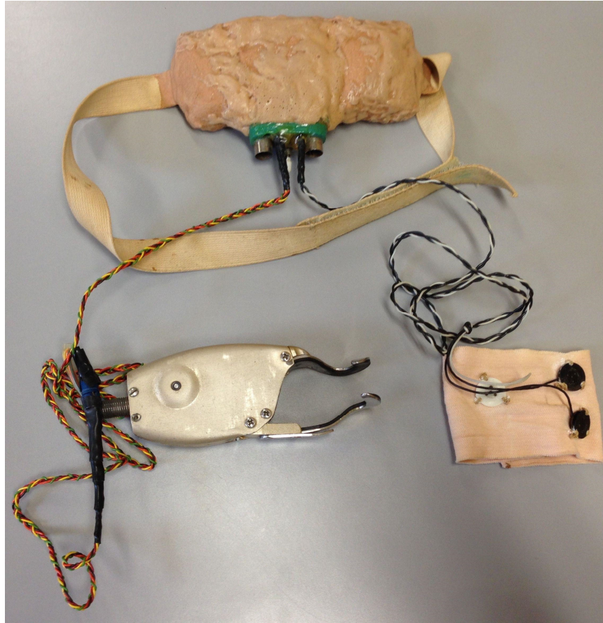
Figure 1: UNB myoelectric control system, 1965, including controller with strap (top), terminal device (left) and electrodes (right).
