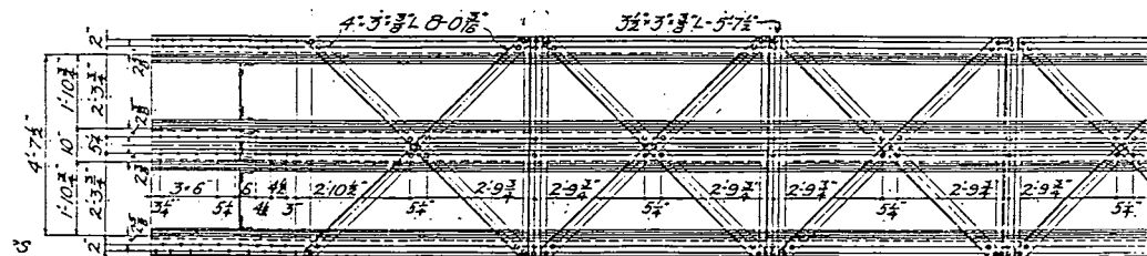
(b) QUEBEC BRIDGE COMPRESSION MEMBER
