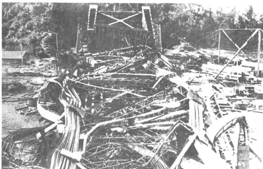
Figure 7(a) Wreckage, looking south [top]; 7(b) looking north
