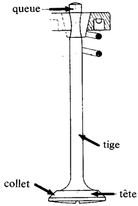
Soupape
