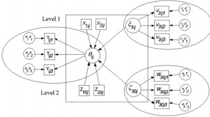
Figure 4. Path diagram of a multilevel IRT model
