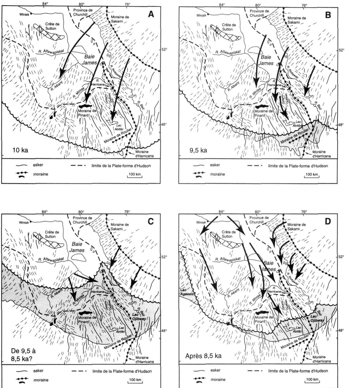
Deglaciation of Abitibi and eastern James Bay basin from about 10 to 8 ka. Arrows indicate ice flow directions (ice margin position is assumed to be reliable for the Lake Ojibway basin only).
