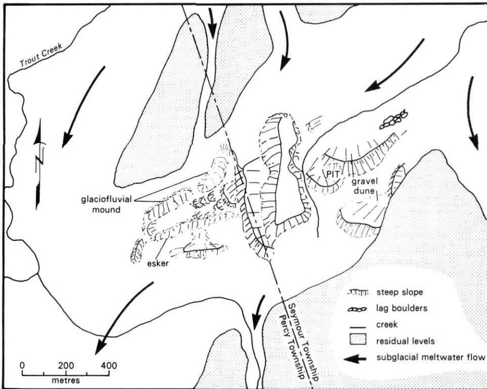
FIGURE 4. Gravel dunes and associated glaciofluvial landforms and sediment, Trout Creek. The pit (also shown in Fig. 3) is the site of most of the sedimentological observation reported in this paper.
