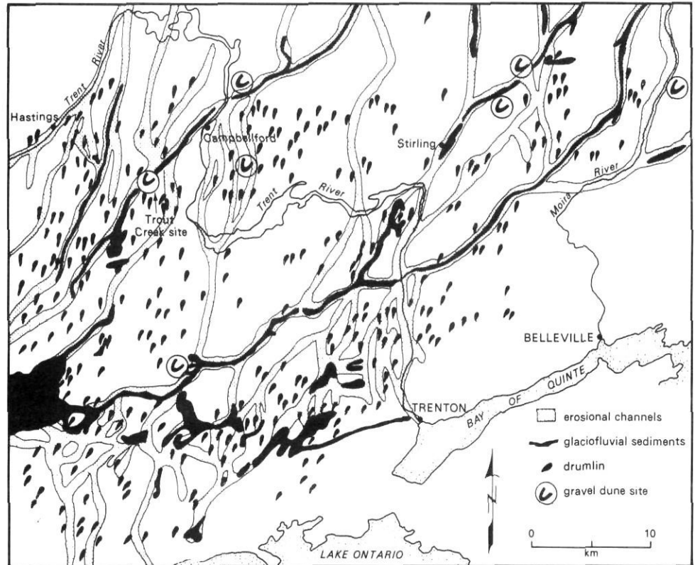
FIGURE 2. Drumlins, tunnel channels (erosional channels), glaciofluvial deposits and gravel dunes sites in the Trenton-Campbellford area.
