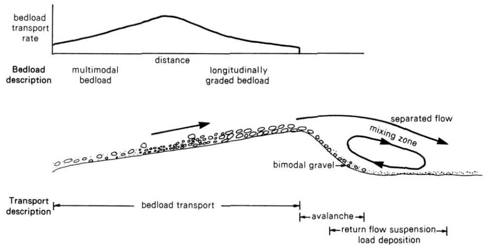
FIGURE 10. Foreset deposition related to longitudinal sorting and bedload transport rates (Iseya and Ikeda, 1987) and suspended sediment deposition from two sources. Note that, at the time of bimodal gravel deposition, suspended sediment is derived mainly from the return flow; direct deposition from the mixing layer is of increased importance during deposition of the bimodal gravel.
