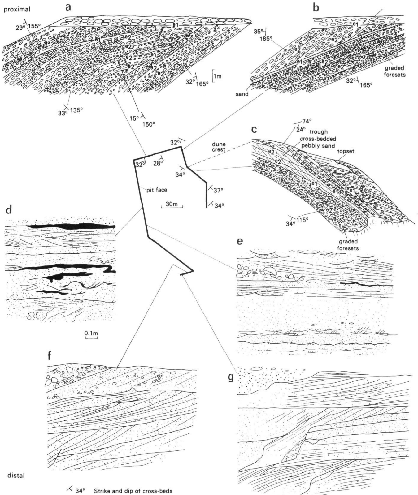
FIGURE 6. Internal structure of a gravel dune and associated produne deposits at Trout Creek. Note the change in scale between the proximal cross-beds in gravel and the sandy or silty (solid black) distal deposits. The e_1 surfaces are major unconformities, the e_2 surfaces are major bedding planes or set boundaries.
