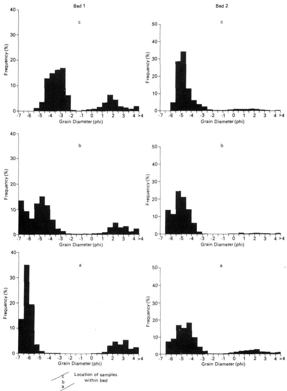
FIGURE 8. Grain size histograms for foreset beds within a gravel dune. Beds a,b,c show an upward fining in the coarse mode and an upward decrease in matrix size (bed 1) or decrease in matrix volume (bed 2).
