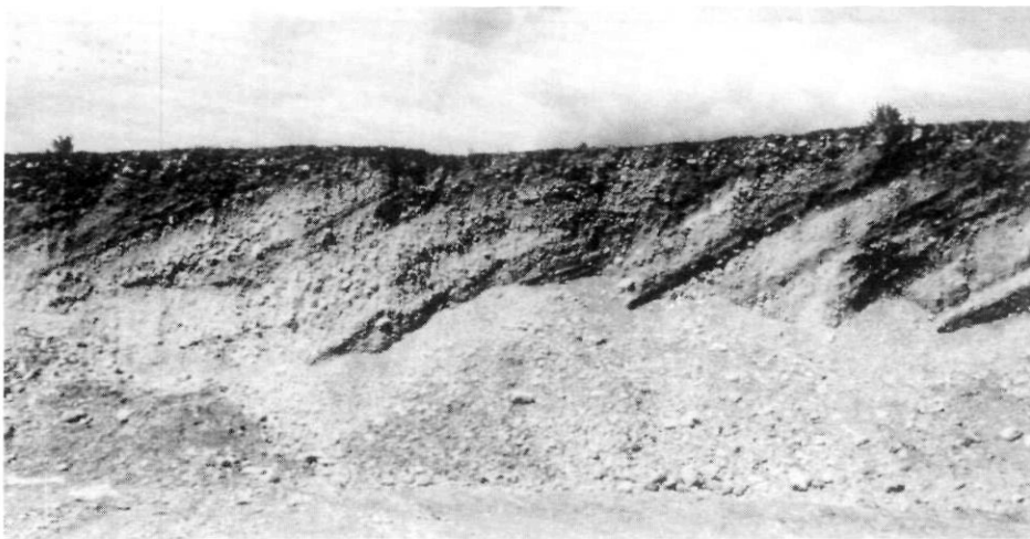
FIGURE 5. Large-scale cross bedding in a gravel dune, Trout Creek. Height of face about 8 m.
