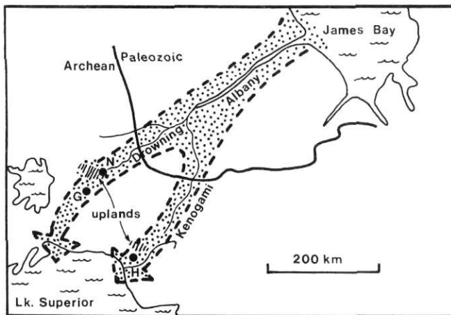
FIGURE 6. Hypothetical location of two zones of rapid ice flow (streaming = stipples) north of Lake Superior, within marginal area of Late Wisconsinan Laurentide Ice Sheet. G = Geraldton; H = Hemlo.
