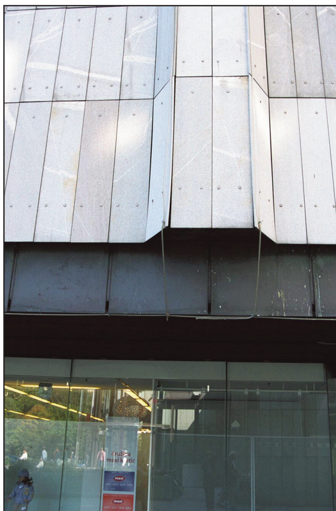
Figure 8. Bowing of granodiorite on a building façade. Photo: Ana Mladenović.
