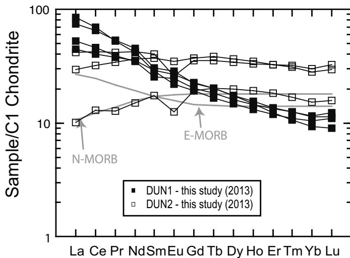
Figure 6. C1-chondrite normalized diagrams of rare earth elements (REE). Normalization values from Sun and McDonough (1989). LH Volc = Lawrence Head Volcanics, NB gb = gabbro sills from the New Bay Formation, DUN1 and DUN2 = blocks from the Dunnage Mélange. Year listed for this study (2003, and/or 2013) refers to the analysis date of each suite of samples.
