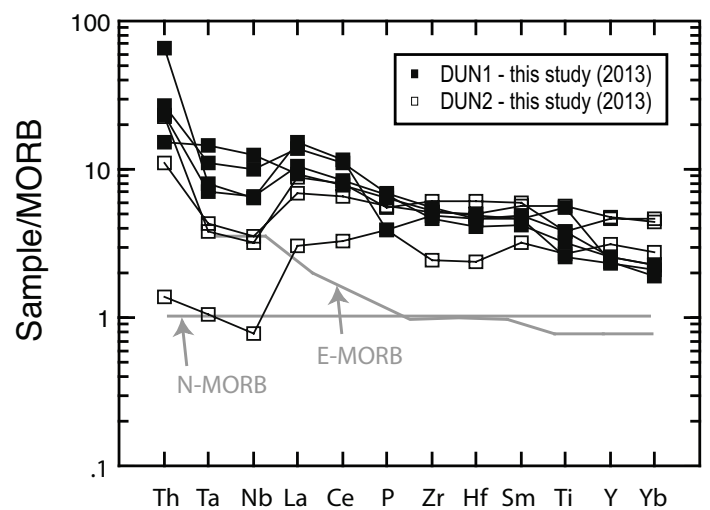
Figure 7. MORB-normalized diagrams of selected trace elements. Normalization values from Sun and McDonough (1989). LH Volc = Lawrence Head Volcanics, NB gb = gabbro sills from the New Bay Formation, DUN1 and DUN2 = blocks from the Dunnage Mélange. Year listed for this study (1982, 2003, and/or 2013) refers to the analysis date of each suite of samples.
