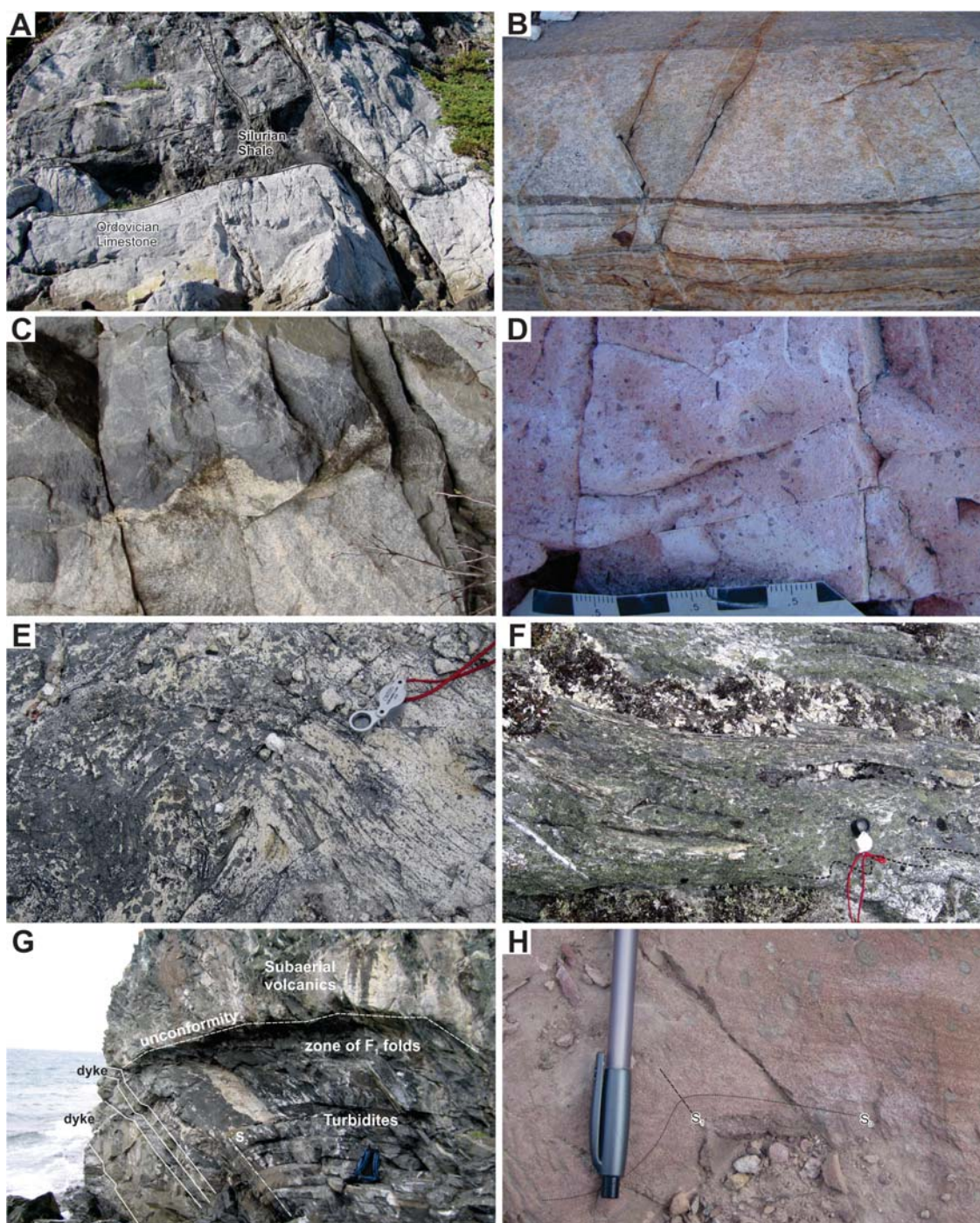
Figure 4. Representative photographs of Silurian rocks along and east of the Red Indian Line. A. Darriwilian limestone blocks in a matrix of Silurian shale of the Joey's Cove mélange at Rogers Cove, New World Island (see Reusch 1987). B. Contact metamorphosed Badger Group turbidites adjacent to the Dawes Pond Granodiorite and Hodges Hill Batholith. Note bedding subparallel to foliation. Nearby outcrops of the Roberts Arm Group preserved evidence for polyphase deformation. C. Twin Lakes phase of the Hodges Hill Batholith displaying scalloped contact between mafic and felsic phases, suggesting they are co-magmatic. D. Pristine hypabyssal quartz-phyric rhyolite of the Dawes Pond Granodiorite. E. Foliated Stony Lake rhyolite deformed into symmetrical folds in hinge of anticline. Folds are accompanied by weak axial planar cleavage. Hand lens for scale. F. Strongly foliated ca. 423 Ma Stony Lake rhyolite. Foliation is tectonic and folded by younger mesoscopic folds containing a weak axial planar cleavage (lower right corner). Hand lens for scale. G. Unconformity between Salinic ( F_1 ) deformed Badger Group turbidites and subaerial volcanic rocks of the Port Albert Formation of the Botwood Group. Turbidites below the unconformity contain a zone of F_1 folds (Karlstrom et al. 1982) and are overlain by a thin conglomerate layer that locally contains pebbles with pre-entrainment cleavage. Both units are folded by NW-verging Acadian(?) structures ( F_3 of Lafrance and Williams 1992). H. Folded and cleaved red beds of Wigwam Formation near the contact with the overlying Stony Lake Formation felsic volcanic rocks.
