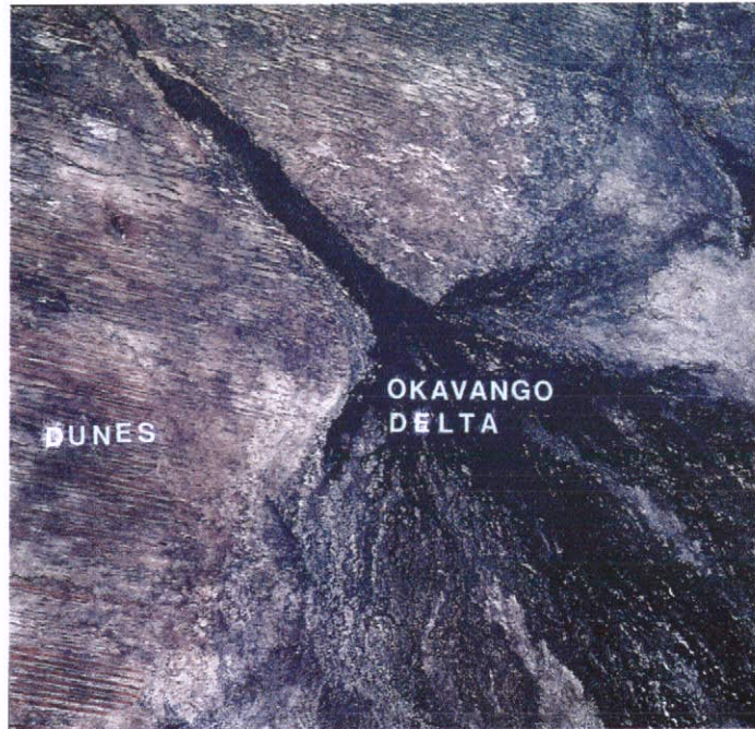
Figure 10 Space Shuttle photograph of the Okavango Oasis/Delta taken in early November 1985 about two months after the arrival of the annual flood. Dark patches are the Okavango River and its tributaries and swamps of the delta plain. The lighter parallel lines in the northwestern part of the photographs are sand dunes stabilized by vegetation (from Strain and Engle, 1996). Published with permission.
