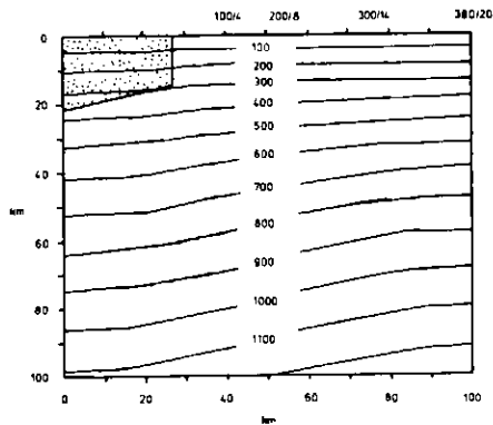
Figure 5 Burial model after 20 Ma of erosion of country rock and deposition upon sediment trough. Figure shows maximum temperature (°C/depth (km)) attained for rocks now exposed at the surface after 20 Ma. The depth/temperature paths followed by these samples are the same as those shown in Figure 7a.
