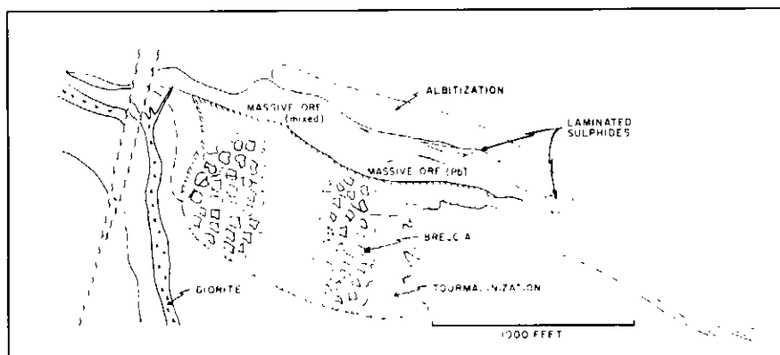
Figure 8 Longitudinal section of the Sullivan deposit showing the marginal, laminated sul-
