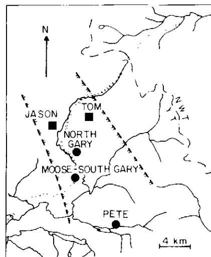
Figure 10 Spatial relationships between Ba (circles), Ba-Zn-Pb-Ag (squares) deposits and the McMillan Pass Graben (modified from Smith, 1978).
