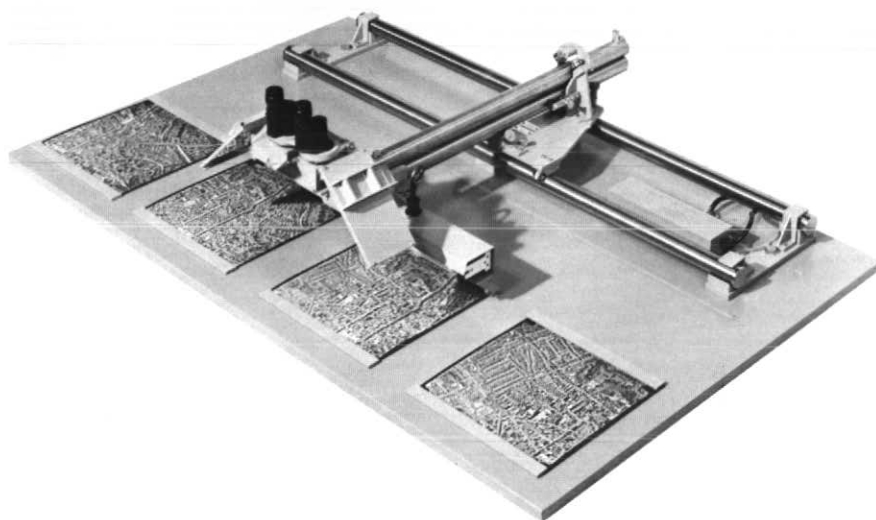
Figure 1 Mirror stereoscope with parallel guidance mechanism. (Courtesy of C.F. Casella and Co. Ltd.)
