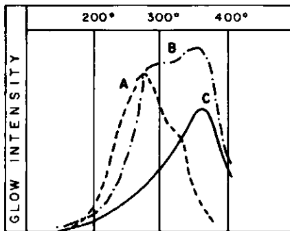
Figure 2 Typical TL glow curves of quartz from three sites in the USSR: (A) Karuküla, Estonia, (B) Lake Tshorkan, Kerch Peninsula, (C) Pasva, Arkhangeisk District.
