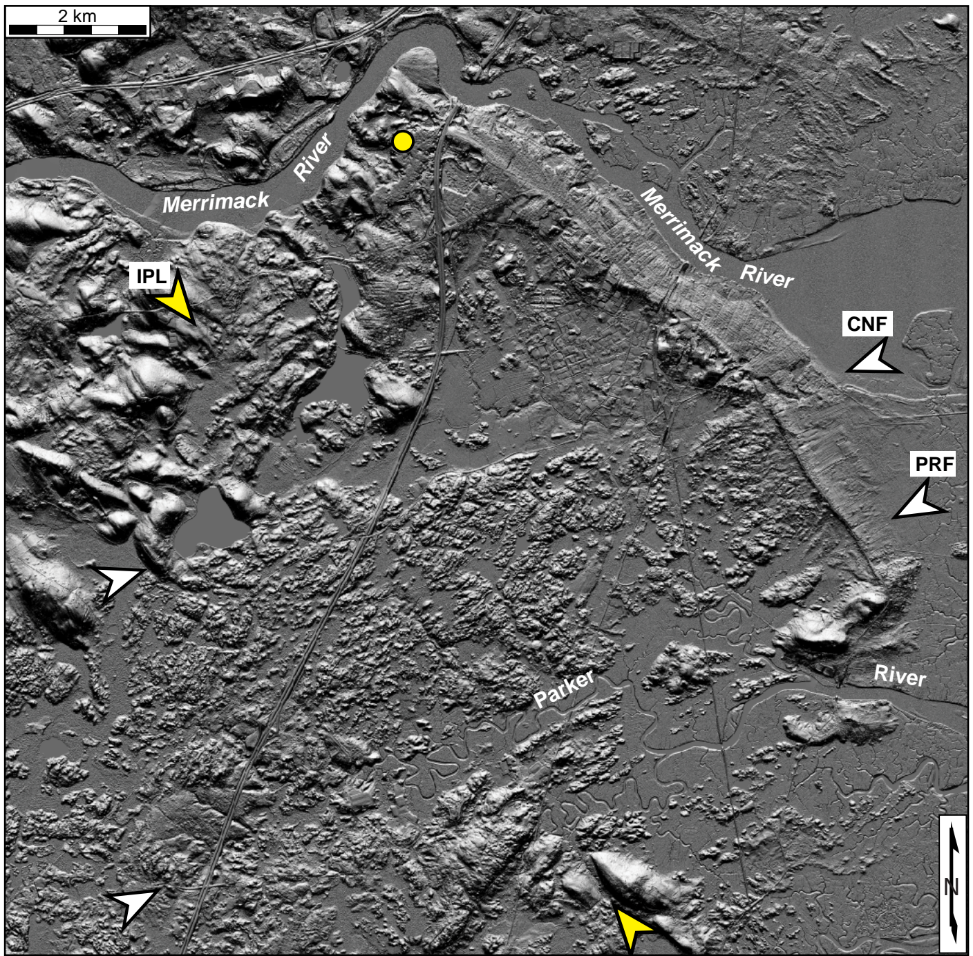
Figure 9. Black and white LiDAR image (illumination angle = 0^\circ ) of the Newburyport, Massachusetts, area. The yellow dot is the location of the epicenter for the 1999 Amesbury earthquake (from Ebel, 2000). The opposing yellow arrows labeled IPL show the location of the Ipswich lineament. The opposing white arrows labeled CNF and PRF show the locations of the Clinton-Newbury and Parker River faults.
