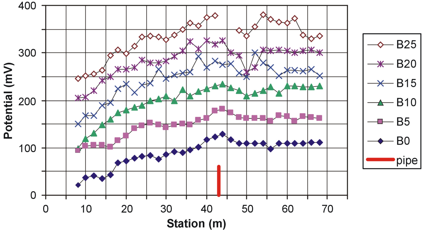
Fig. 8. SP profiles of Grid B (Fig. 1) taken on different days in September, 2005. Missed readings on Line B25 correspond to a large puddle on the road.
