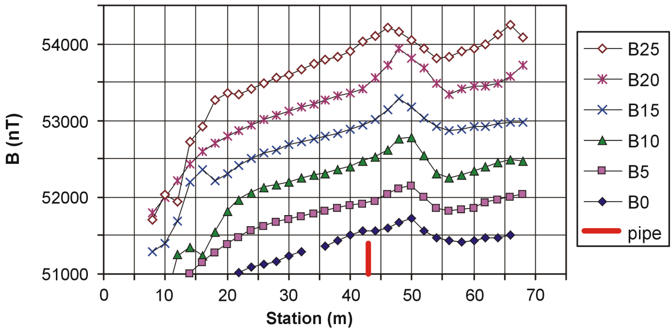
Fig. 9. Profiles of total magnetic field on Grid B, taken on various days in September, 2005. Values on vertical axis apply to profile B0. Each overlying profile is further offset by 500 nT.
