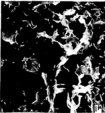
Figure 3 - Scanning electron micrograph of freeze-dried grundite illite floccules. Flocculated in salt water ( \text{Na Cl } 1\text{ gm/l.} ) x 6000.
