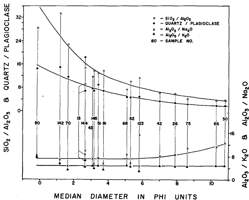
FIGURE 8 - Variation of \text{SiO}_2/\text{Al}_2\text{O}_3 ; \text{Al}_2\text{O}_3/\text{K}_2\text{O} ; \text{Al}_2\text{O}_3/\text{Na}_2\text{O} ; and quartz/feldspar ratios with median diameter for sediment samples from the Scotian Shelf.
